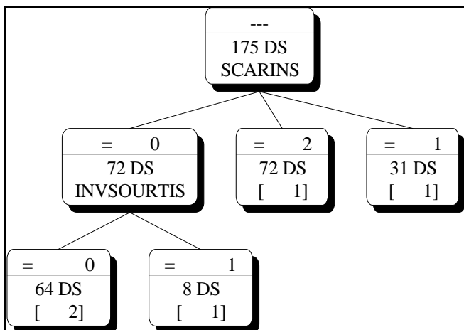
Figure 3. Decision Tree with Feature Subset Selection
